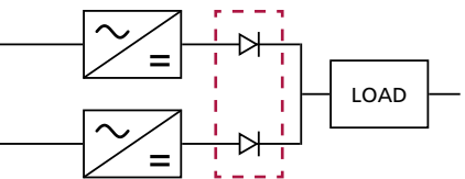
Application case 2: If a power source fails, the second power source automatically takes over the supply of power.
