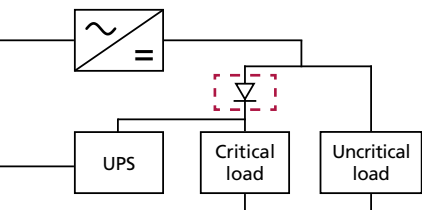
Application case 1: Decoupling of critical paths to maintain the function of important components for longer.
