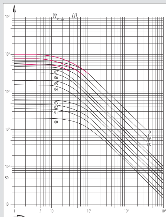
Friction switching frequency Type N, H, D
