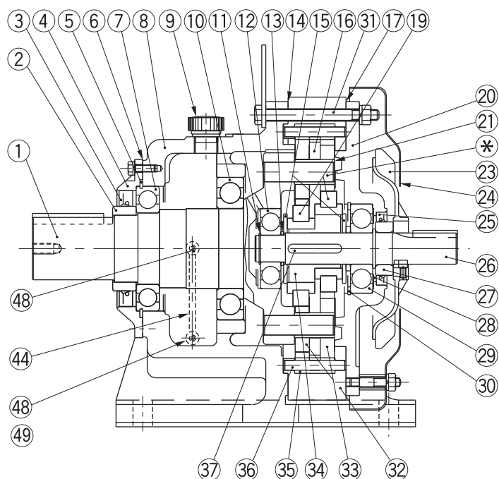
Typ CHH (Horizontal, Reducer) Single Reduction (Example: Frame size 6175)
