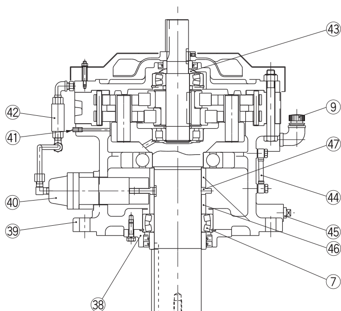
Typ CVV (Vertical, Reducer) Single Reduction (Example: Frame size 6225)
